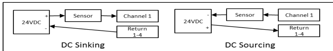
Figure 2. Typical External Wiring Application for the Model 2589-B
