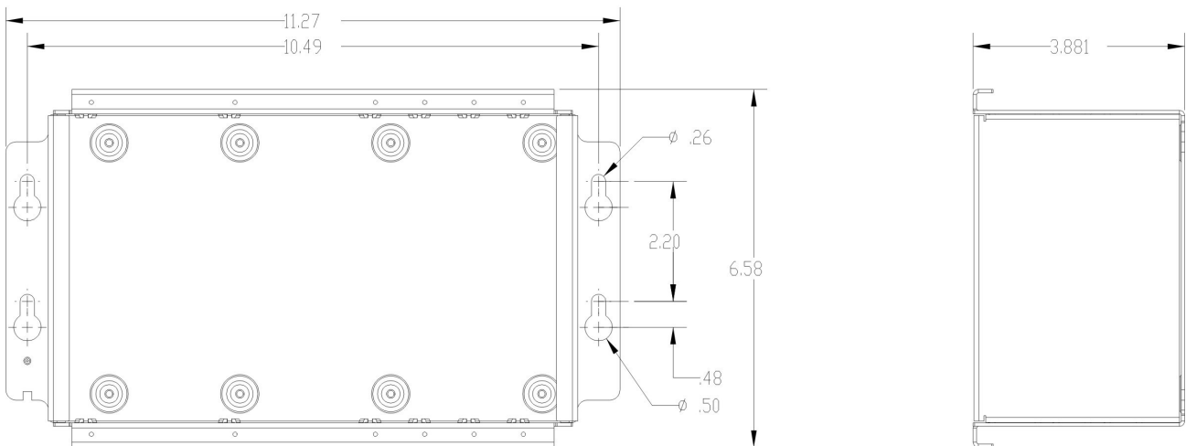
2500C-R4 Mounting Dimensions Mounting Hole Dimensions
