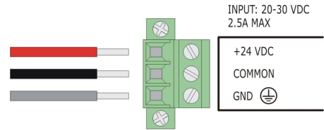
User Supplied Power Input Wiring Diagram
